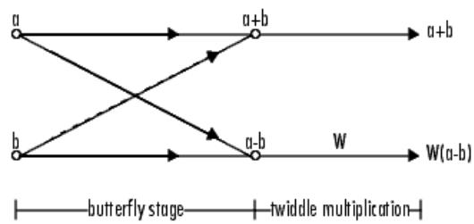
Decimation-in-frequency IFFT
