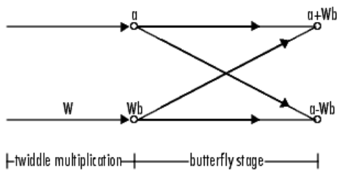
Decimation-in-time IFFT
